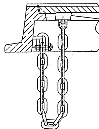
鎖取付部拡大図 (Sc=1/3)
